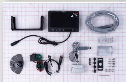
CAMERA SYSTEM- REAR MOUNT W/7" COLOR LCD MONITOR
