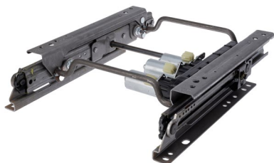
BASE ONLY, DRVR- SIDE 6-WAY PWR W/O SWITCH KIT (1193029)
